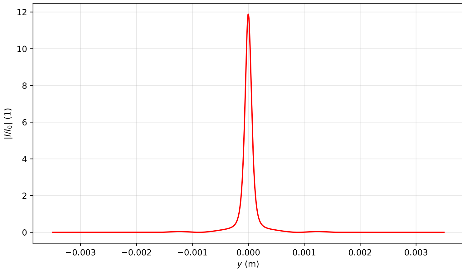
Intensity profile I(x=0, y, z=1.911)/I_0 , P_{in}=2.5P_{cr} , artificial time
